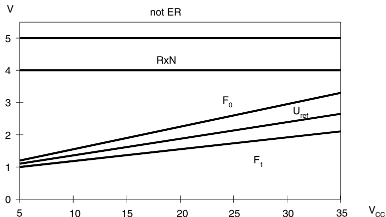
Figure 7-1. Comparator Thresholds
